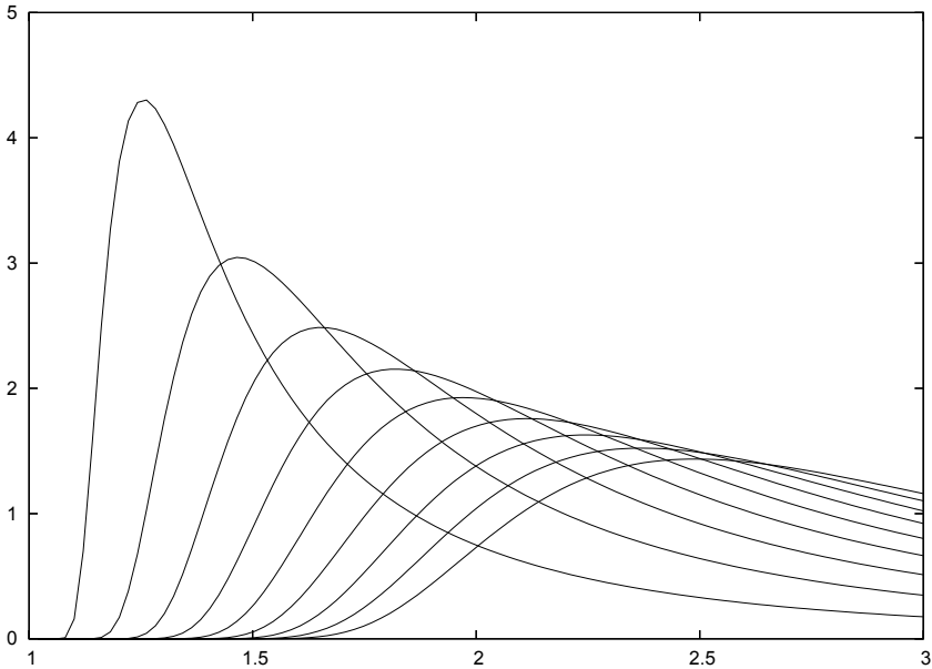
Figure 1. Energy density \tilde{\epsilon} = a\epsilon as a function of \tilde{r} = r/a for \tilde{\alpha} = \alpha/a = 1, \dots, 9 . The first curve on left corresponds to \tilde{\alpha} = 1 , whereas that the last curve on right corresponds to \tilde{\alpha} = 9 .
