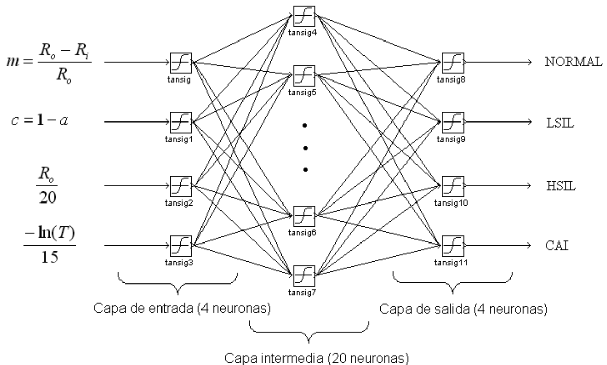
Figura 5. Red neuronal artificial.
