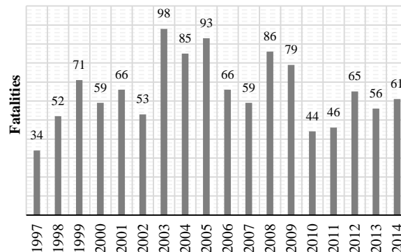
Figure 2. Lightning fatalities in Colombia. Source. Authors.
