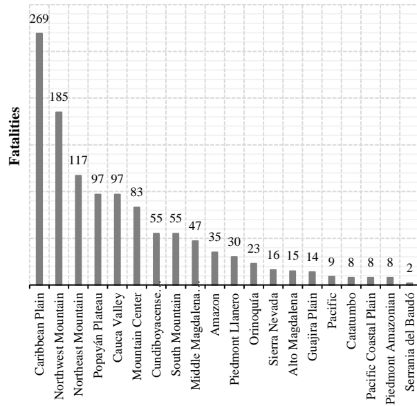
Figure 3. Lightning fatalities in the natural sub-regions of Colombia. Source. Authors.
